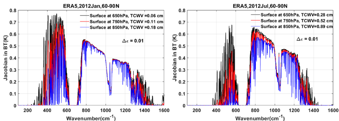
Fig. 8. Sensitivity of BT at TOA to surface emissivity change of 0.01 at different surface elevations. The ERA5 profile averaged over the Arctic ( 60^\circ – 90^\circ\text{N} ) is used. (left) January and (right) July 2012. The TCWV for different surface elevations are labeled in each panel.
