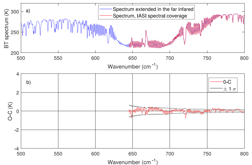
Fig. 9. (a) IASI assessment of spectroscopy accuracy for the core of the \nu_2 \text{ CO}_2 band. (b) Results based on observations (O) minus calculations (C) in for a set of IASI spectra [whose average is shown in (a)] recorded in 2014 over the Global Climate Observing System Reference Upper-Air Network (GRUAN) Manus validation station. The figure is intentionally extended down to 500 \text{ cm}^{-1} to highlight that portion of the \nu_2 \text{ CO}_2 band that is currently not covered by meteorological satellite missions.
